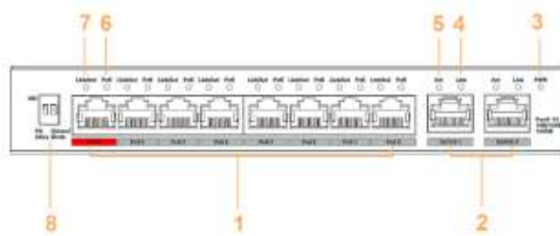
Figure 2-1 Front panel
