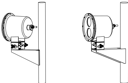
Figure 2-1 Pole Mounting
