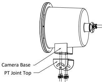
Figure 2-3 PT Joint Top Installation
