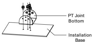
Figure 2-4 PT Joint Bottom Installation
