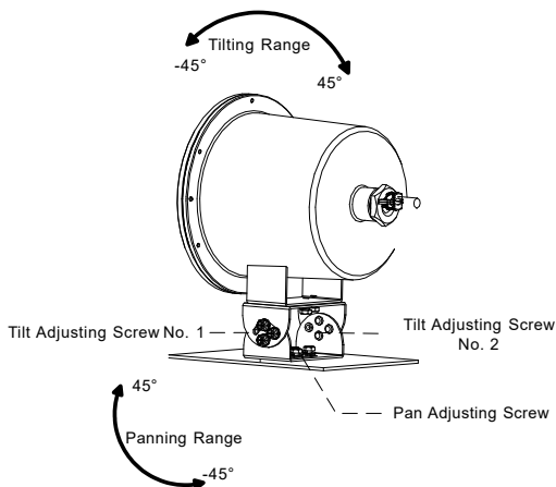
Figure 2-1 2-Axis Adjustment
