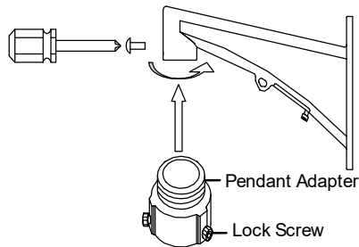
Figure 3-14 Pendent Adapter
