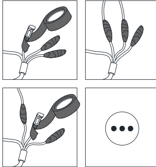
Figure 3-1 Waterproof Cable
