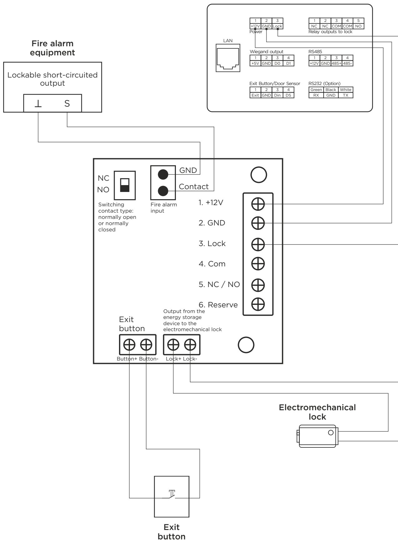
Diagram of connection of outdoor panels using an electromechanical lock connected from an uninterruptible power supply
