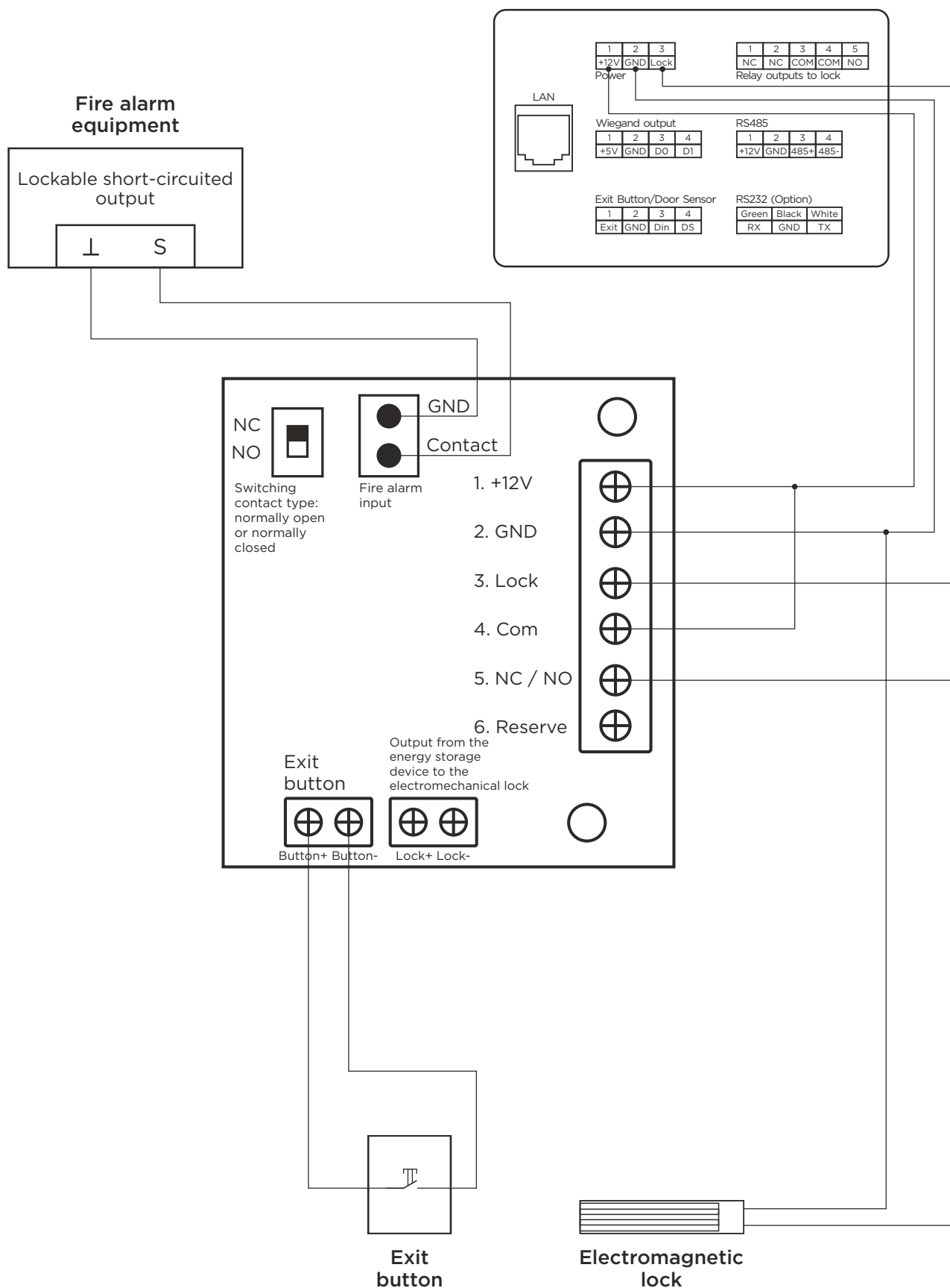
Connection diagram of outdoor panels using an electromagnetic lock connected from an uninterruptible power supply
