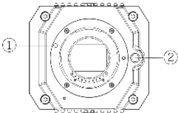
Figure 9-2 Front panel
