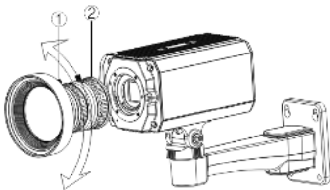
Figure 9-3 Lens installation (2)
