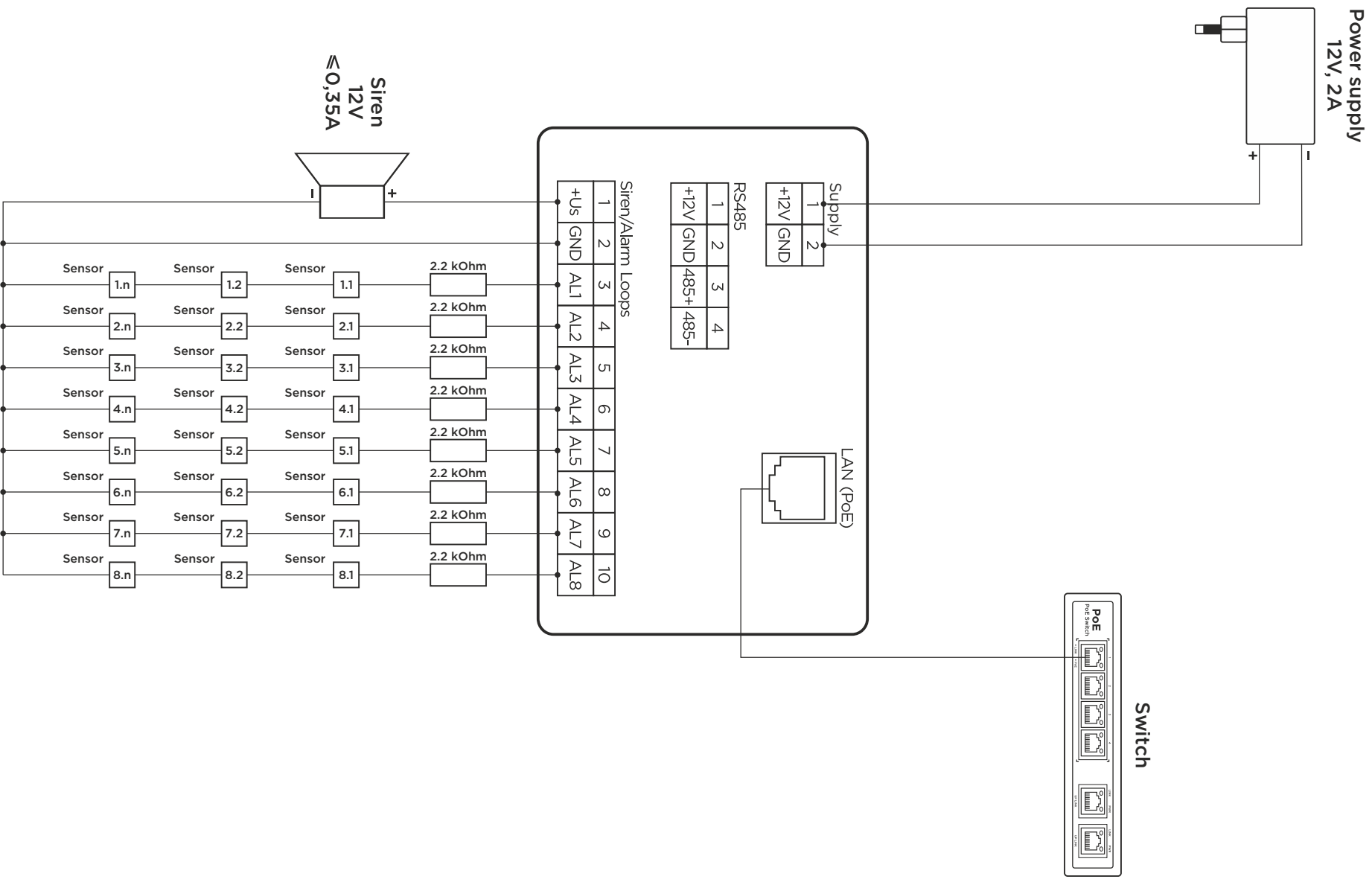
Wiring diagram for security alarm sensors with NC - normally closed contact types
