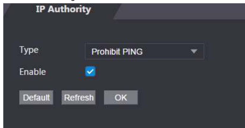
Figure 3-13 Prohibit PING
