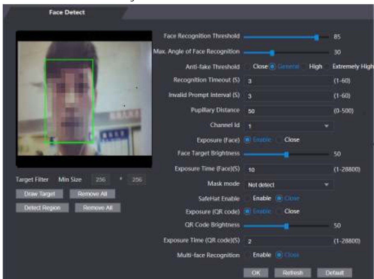
Figure 3-8 Face detect
