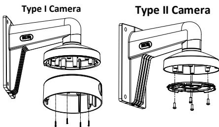
Figure 2-6 Attach the Base Plate to the Mount
