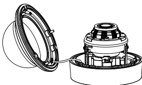
Figure 2-8 Remove the Bubble and the Black Liner
