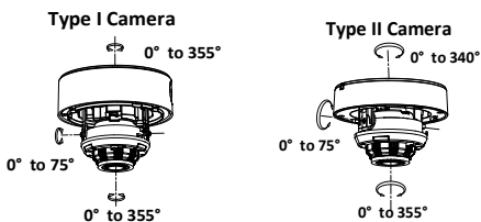
Figure 2-4 3-Axis Adjustment
