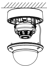
Figure 2-11 Fit the Black Liner Back
