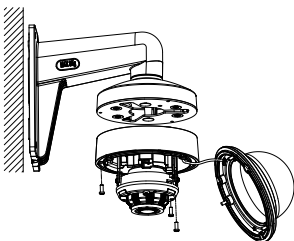
Figure 2-14 Attach the Back Box to the Mount
