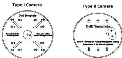
Figure 2-1 The Drill Template
