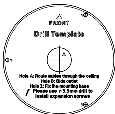
Figure 2-7 The Drill Template
