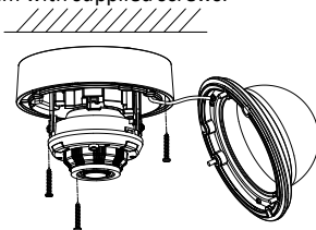
Figure 2-9 Attach the Back Box
