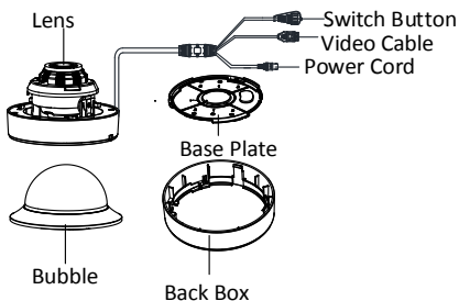
Figure 1-2 Overview of Type II Camera
