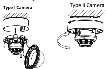
Figure 2-3 Fix the camera to the Ceiling
