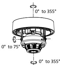
Figure 2-10 3-Axis Adjustment
