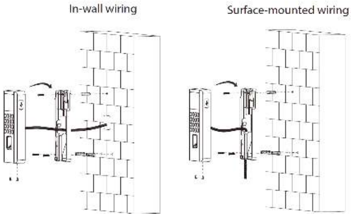
Figure 2-7 Wall mount
