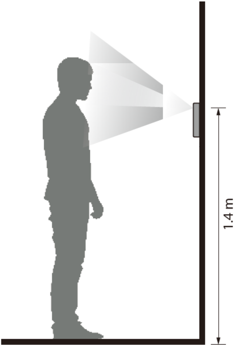
Figure 2-3 Installation height requirement
