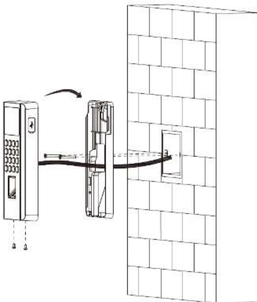
Figure 2-8 86 box mount
