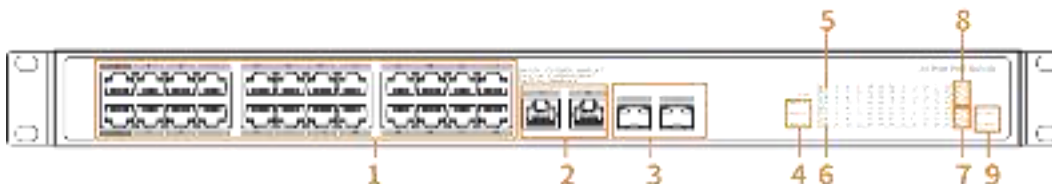
Figure 2-3 Front panel
