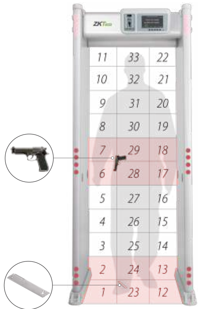
▲ Detection area
