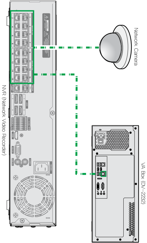
Example 4 : VA Box Connection Diagram without PoE Switch
