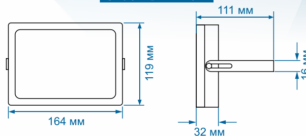
SkatLED LL-30m
