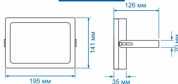
SkatLED LL-30m
