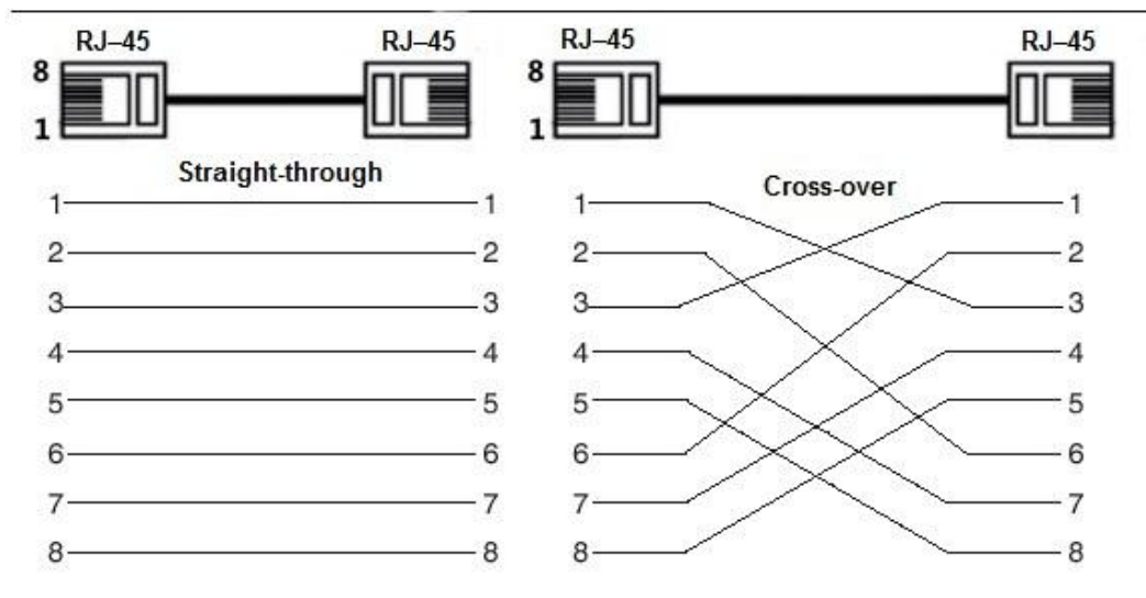
Figure 3-3 Pin description
