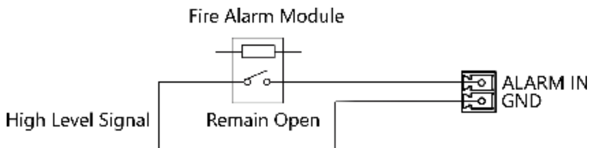
Figure 4-6 Remaining Open
