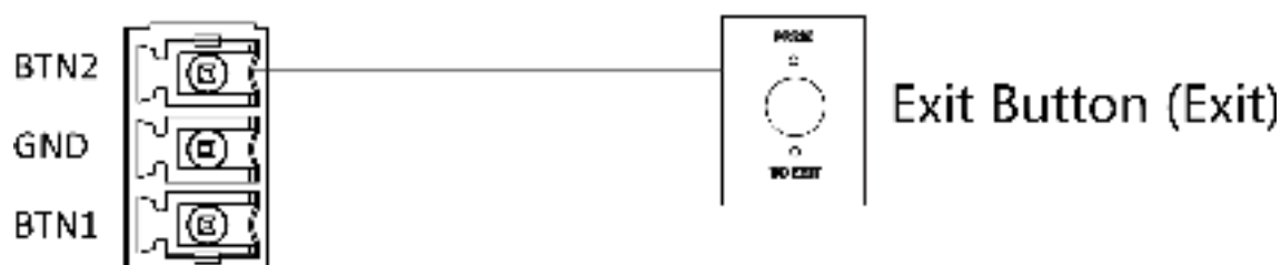
Figure 4-9 Exit Button Wiring (Exit)
