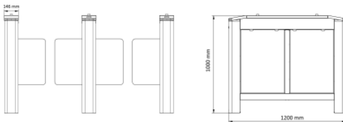
Figure 2-1 Dimension
