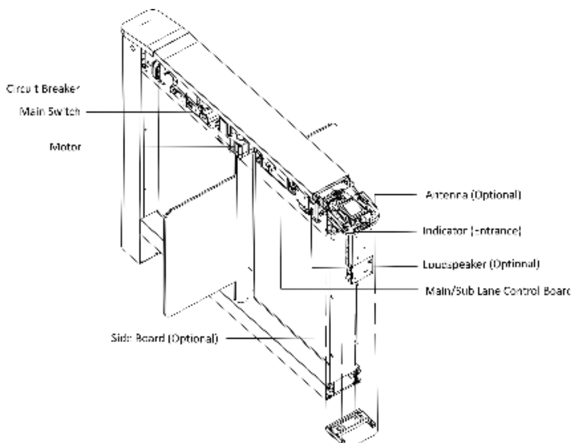
Figure 4-1 Components Diagram
