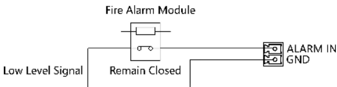
Figure 4-7 Remaining Closed
