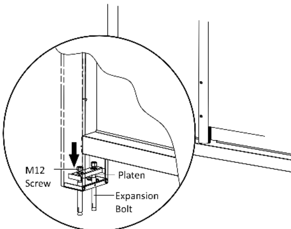
Figure 3-3 Platen
