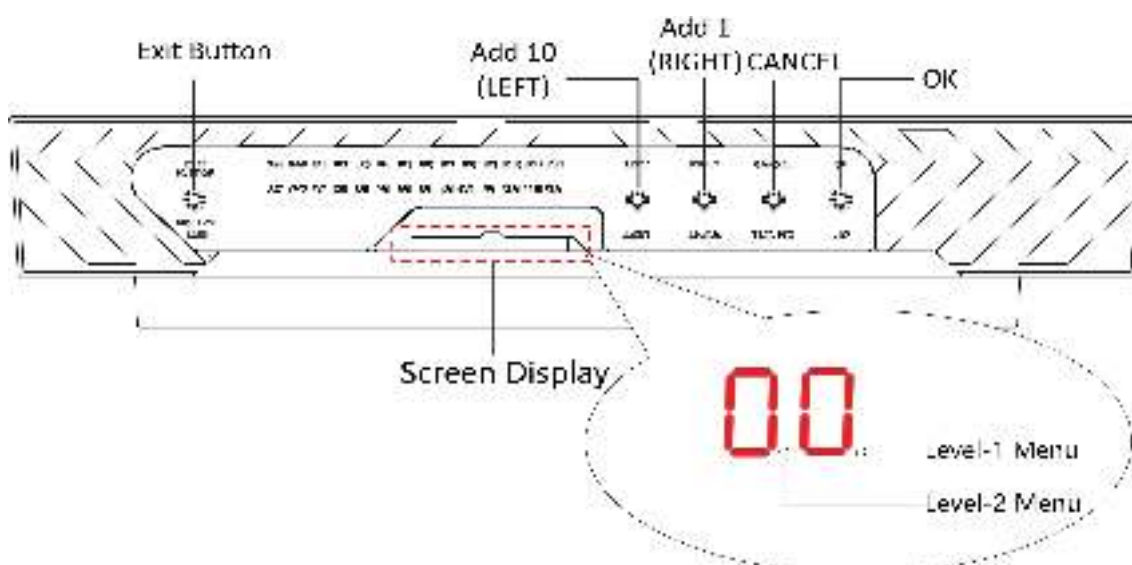
Figure 4-10 Button
