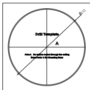
Figure 2-56 Drill Template
