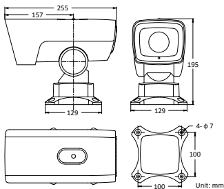
Figure 2-50 Base-mounted PTZ Bullet Camera
