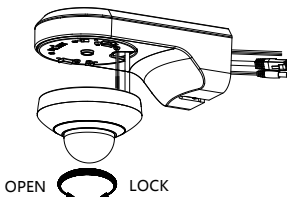
Figure 2-19 Install the Camera
