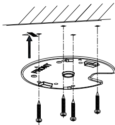
Figure 2-14 Fix the Installation Plate
