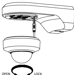
Figure 2-25 Secure DE2xxx Series PTZ Camera
