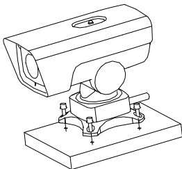
Figure 2-53 Install Base-mounted Camera
