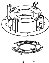
Figure 2-46 Fix the Base Plate to In-ceiling Bracket
