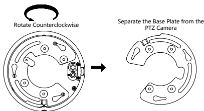
Figure 2-55 Separate the Base Plate from the PTZ camera
