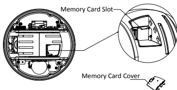
Figure 2-12 For 4× Camera Module
