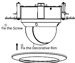
Figure 2-59 Assemble the Decorative Rim
