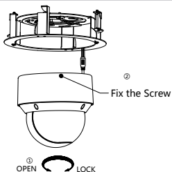
Figure 2-58 Fix the Camera
