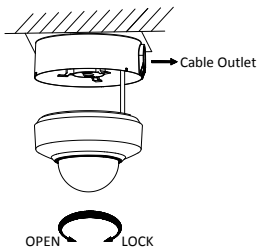
Figure 2-41 Fix the Camera
