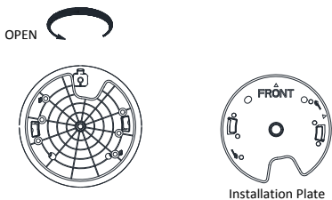
Figure 2-13 Remove the Installation Plate
