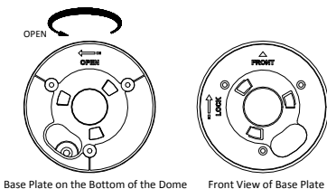
Figure 2-22 Base Plate for DE2xxxI Series (IR) PTZ Camera
