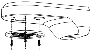
Figure 2-23 For DE2xxx Series PTZ Camera
