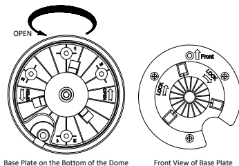
Figure 2-37 For DE2xxx Series PTZ Camera
