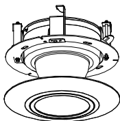
Figure 2-48 Assemble the Decorative Rim
