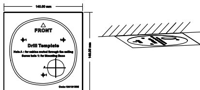
Figure 2-42 Attach the Drill Template
