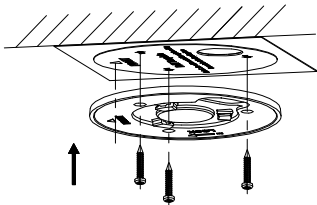
Figure 2-35 For DE2xxxI Series (IR) PTZ Camera
