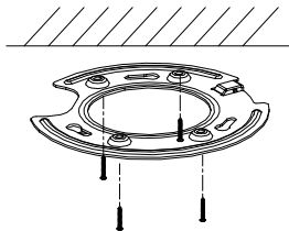
Figure 2-43 Fix the Base Plate
