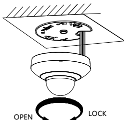
Figure 2-15 Fix the Camera
