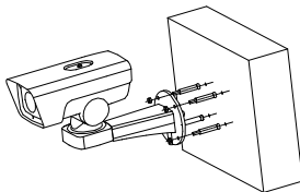
Figure 2-52 Install the Wall-mounted PTZ Bullet Camera
