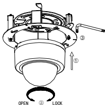
Figure 2-47 Fix the Camera
