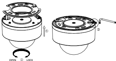
Figure 2-44 Fix the Camera
