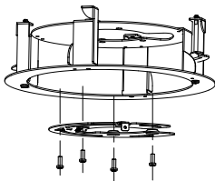
Figure 2-57 Fix the Base Plate to In-ceiling Bracket
