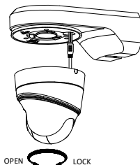
Figure 2-26 Secure DE2xxxI Series (IR) PTZ Camera
