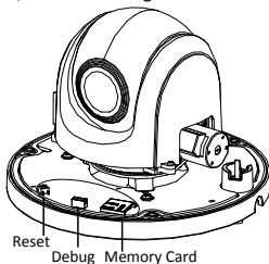
Figure 2-8 DE3xxx Series PTZ Camera
