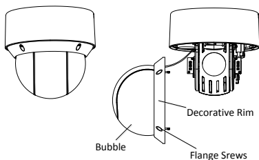
Figure 2-10 Remove the Bubble and the Decorative Rim
