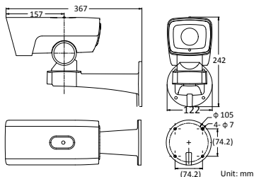
Figure 2-49 Wall-mounted PTZ Bullet Camera
