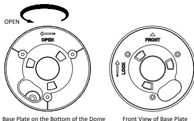
Figure 2-38 For DE2xxxI Series (IR) PTZ Camera
