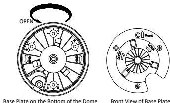
Figure 2-21 Base Plate for DE2xxx Series PTZ Camera
