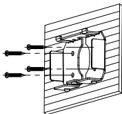
Figure 2-18 Install the Bracket Base
