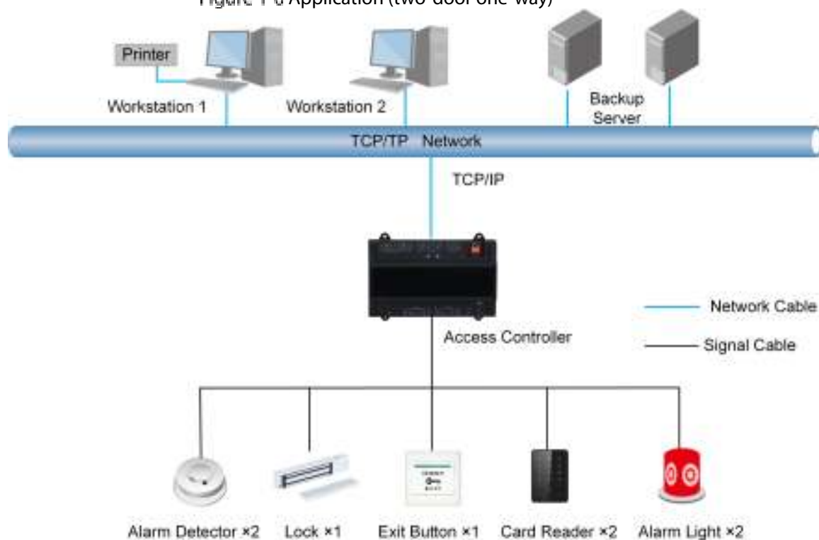
Figure 1-8 Application (two-door one-way)
