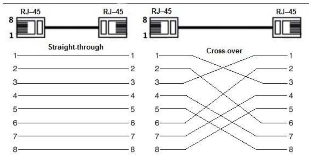
Figure 3-3 Pin description
