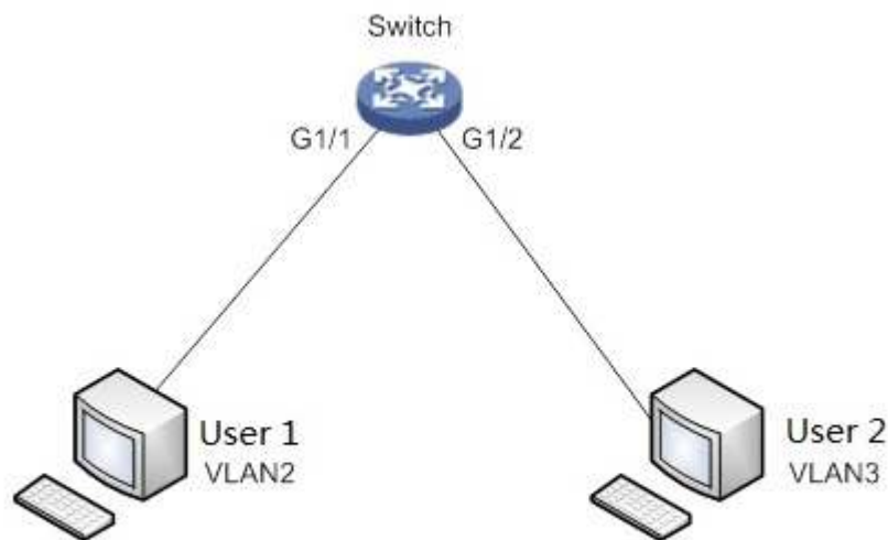
Figure 4-2 VLAN networking
