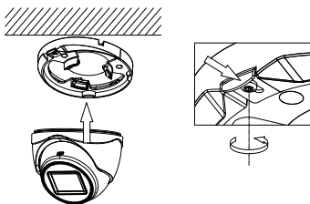
Figure 2-11 Install the Camera
