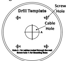
Figure 2-13 Drill Template of the Junction Box
