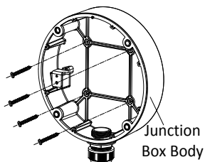
Figure 2-15 Secure the Junction Box's Body on Ceiling
