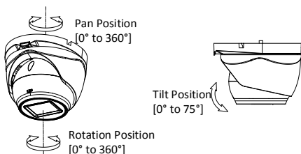
Figure 2-12 3-axis Adjustment
