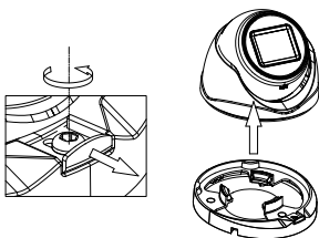
Figure 2-9 Remove the Clip Plate
