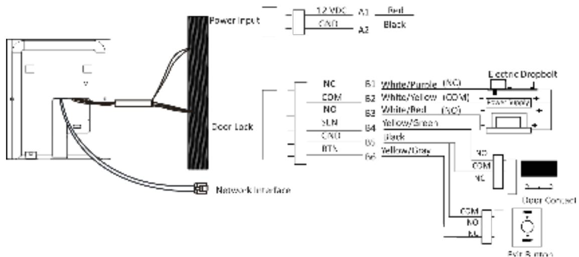
Figure 4-1 Device Wiring
