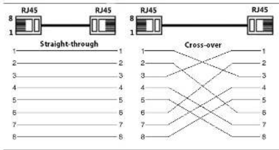
Figure 4-3 Cable connection
