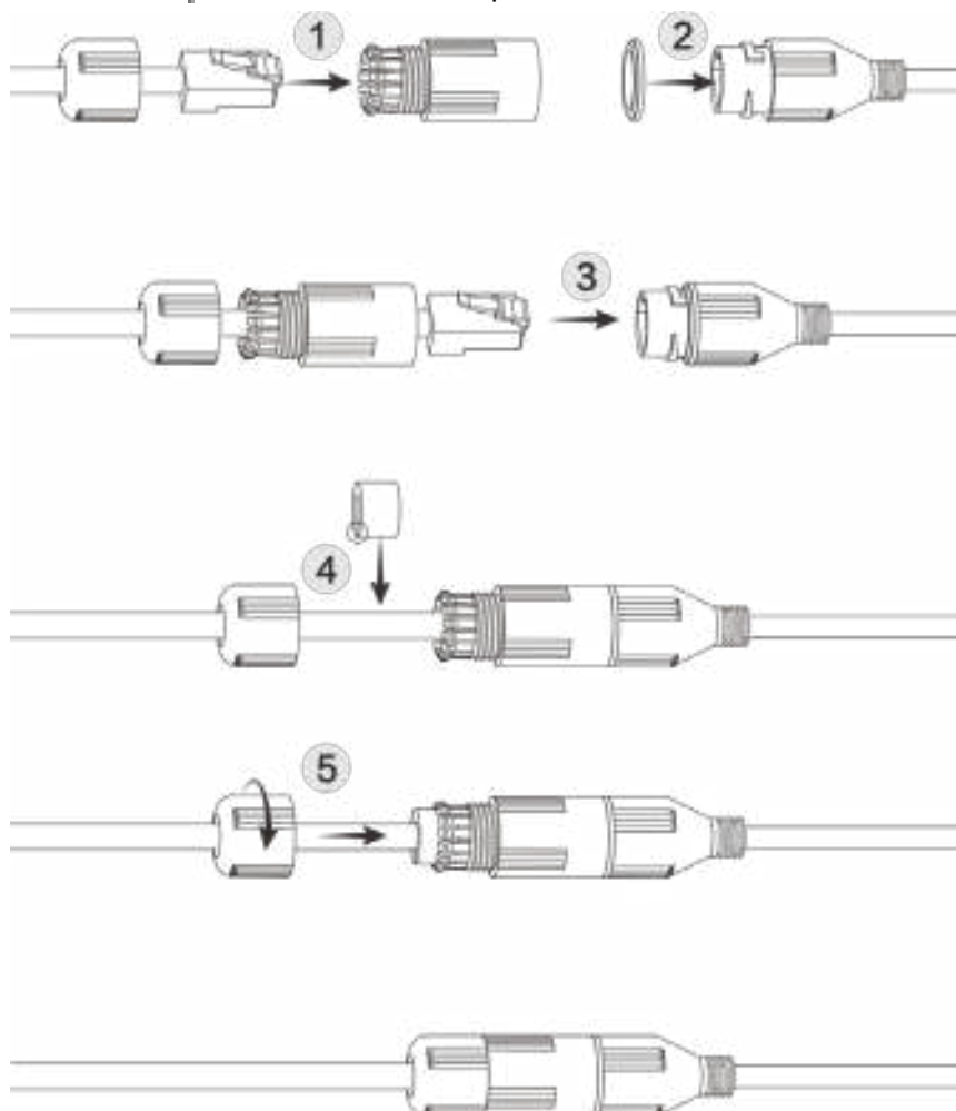
Figure 3-6 Install the waterproof connector
