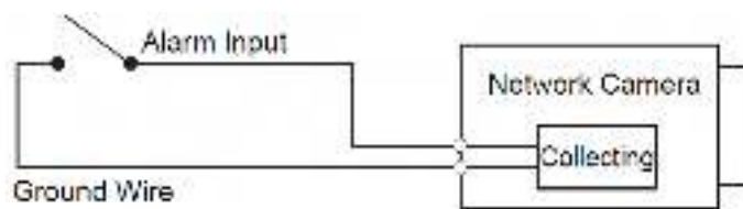
Figure 1-2 Alarm input
