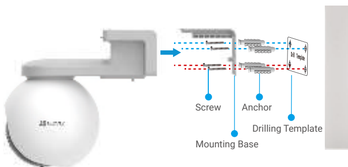
Fig. 2 Wall Mount
