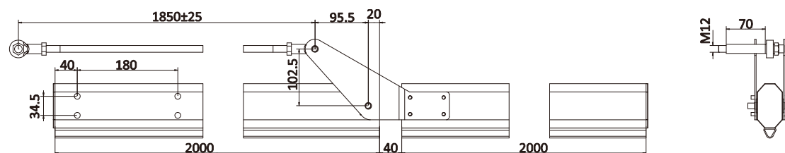
DS-TMG004-5(4m) (Left)/TMG513-L
