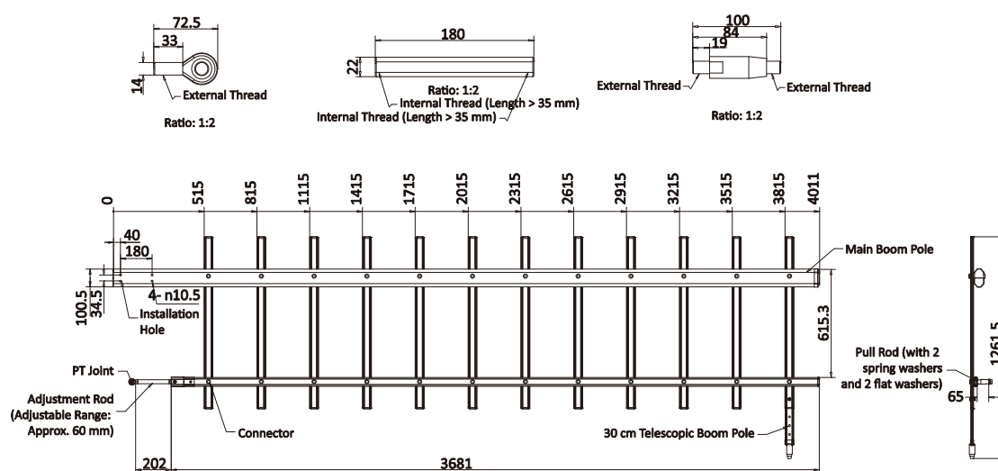
DS-TMG004-5(4m) (Right)/TMG513-R
