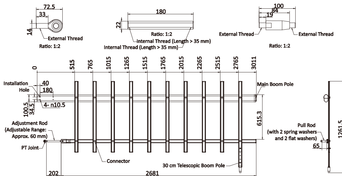
DS-TMG004-5(4m) (Right)/TMG513-R
