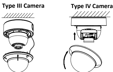
Figure 2. 13 Finish the Installation
