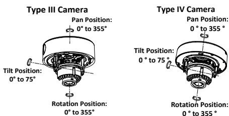
Figure 2. 12 3-axis Adjustment
