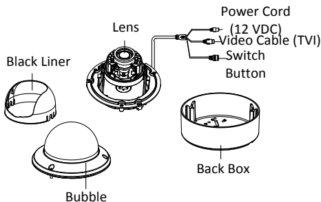
Figure 1. 3 Type III Camera Overview
