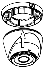
Figure 2. 7 Secure the Camera with Mounting Base
