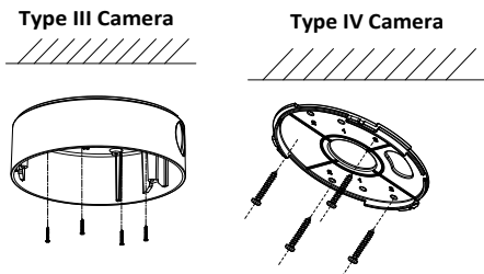
Figure 2. 10 Attach the Back Box/Base Plate
