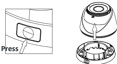
Figure 2. 5 Disassemble the Camera
