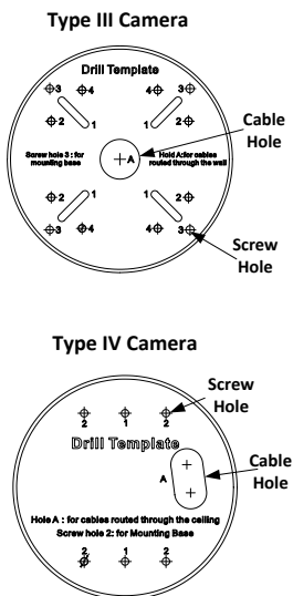
Figure 2. 9 The Drill Template
