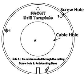
Figure 2. 4 Drill Template
