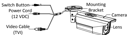
Figure 1. 1 Type I Camera Overview
