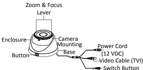
Figure 1. 2 Type II Camera Overview
