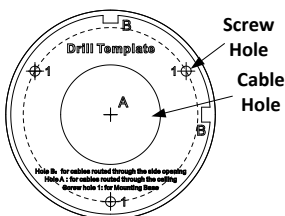
Figure 2. 1 Drill Template
