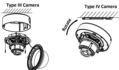
Figure 2. 11 Fix the Camera to the Ceiling
