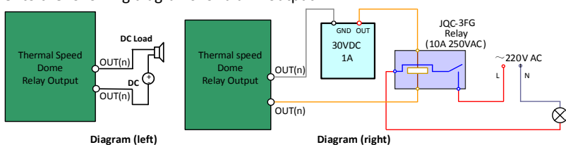
Figure 2-4 Alarm Out Connections
