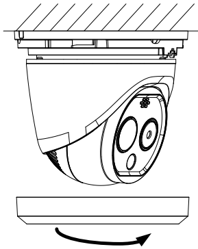
Figure 3-9 Mount the Ring
