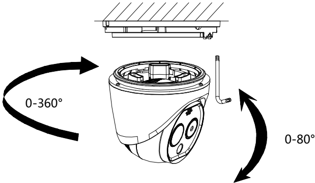
Figure 3-7 Mount the Camera Body
