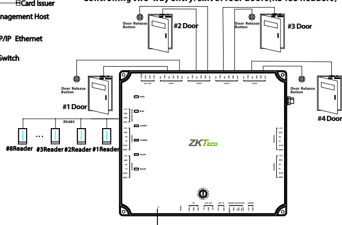
Controlling two-way entry/exit of four doors (RS485 Readers)
