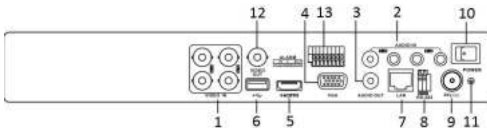
Figure 1-9 Rear Panel of DS-7200HUHI-K/P
