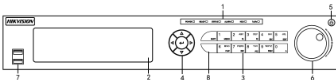
Figure 1-2 Front Panel
