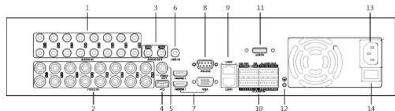
Figure 1-25 Rear Panel of DS-8100HTHI-K8
