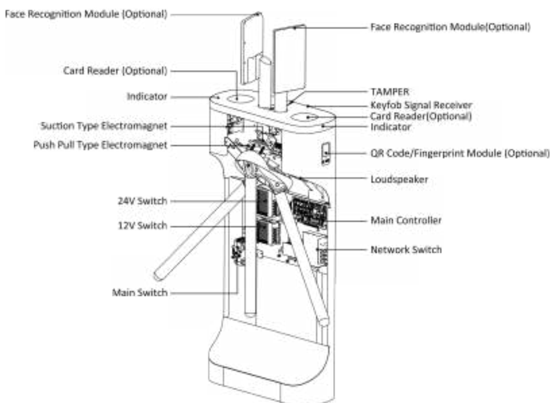
Figure 4-1 Components Diagram 1
