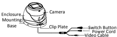
Figure 1-2 Overview of Type II Camera
