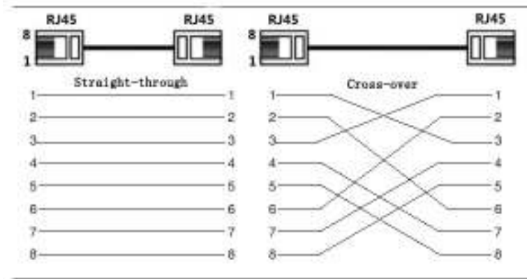
Figure 4-5 Cable connection
