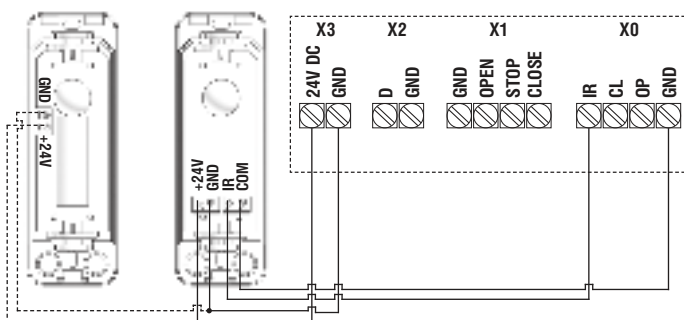
SHAFT 60/120
