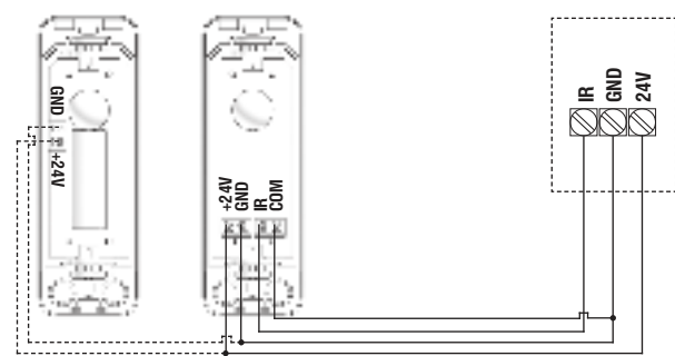
SECTIONAL 800PRO/1000PRO/1200
