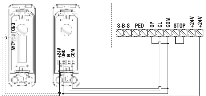
SWING 2500/3000/5000, ARM 320
