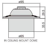
IN CEILING MOUNT DOME
