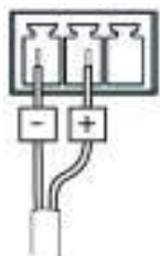
DC power input 24–34 V DC AXIS P5532: max 15 W AXIS P5534: max 17 W
