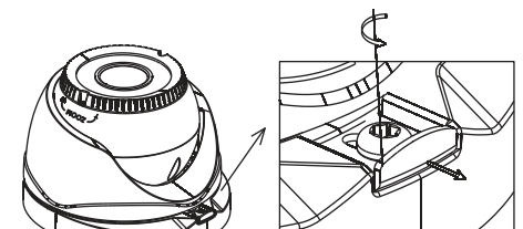
Figure 2-12 The Lock Screw
