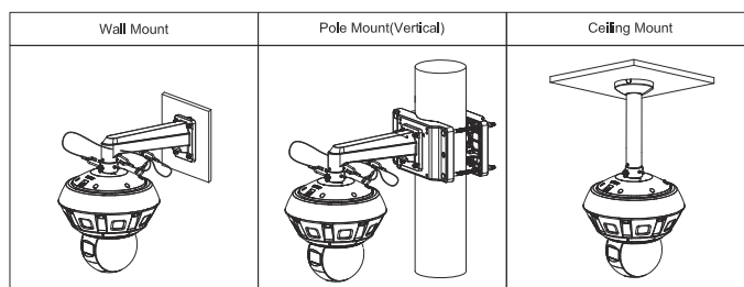
DH-PFA153-SG Pole-mounted bracket
