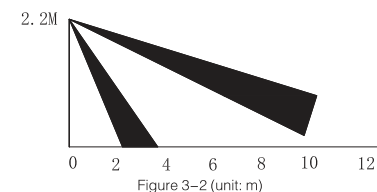
Figure 3-2 (unit: m)
