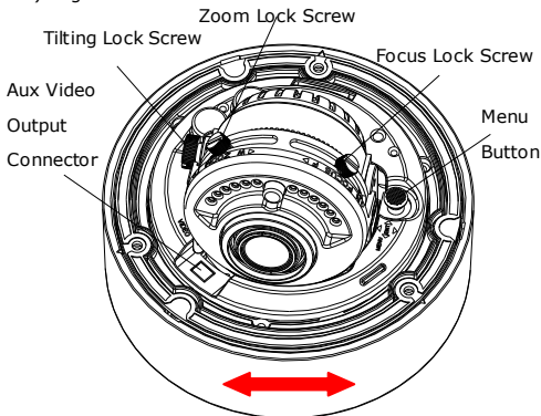
Figure 2-17 Lens Adjustment
