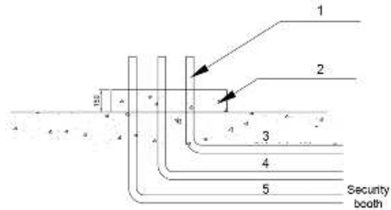
Figure 4-2 PVC pipe layout (mm)
