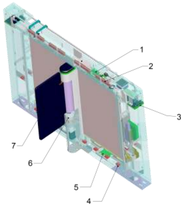
Figure 3-4 Inner components
