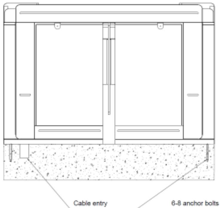
Figure 4-8 Cable entry
