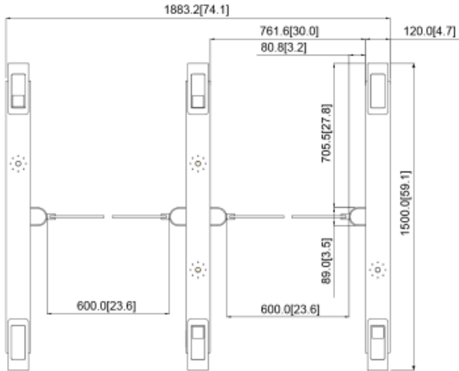
Figure 4- Installation drawings (mm [inch])
