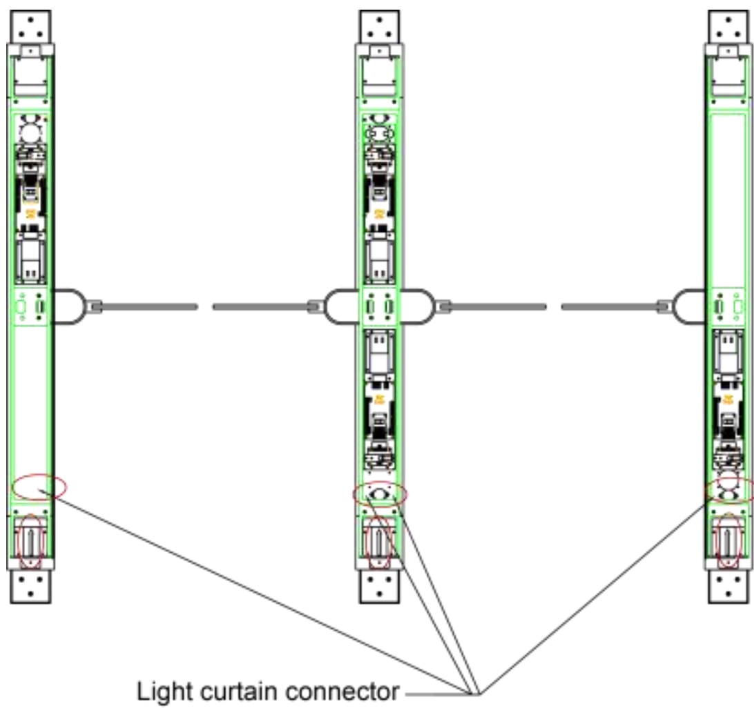
Figure 4-12 Light curtain connector location
