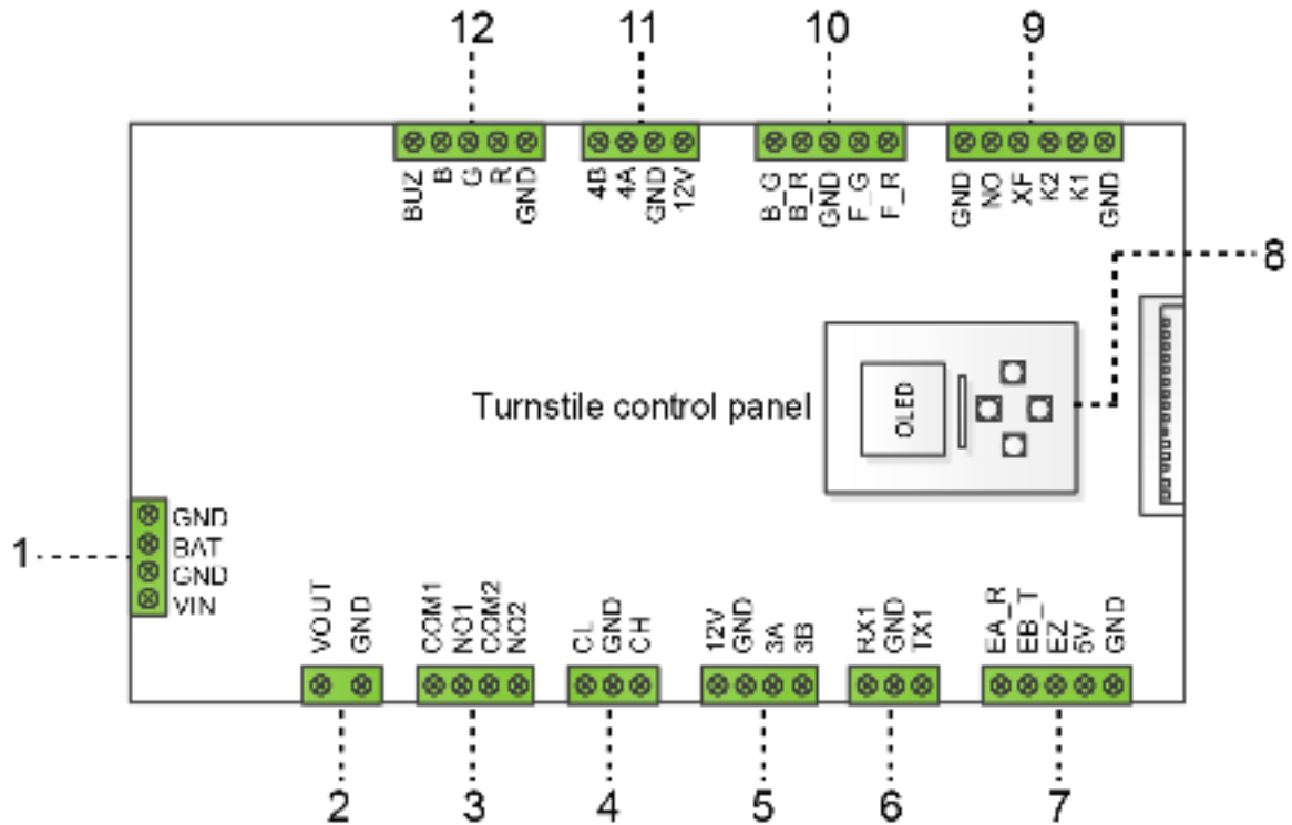
Figure 5-1 Turnstile control panel port
