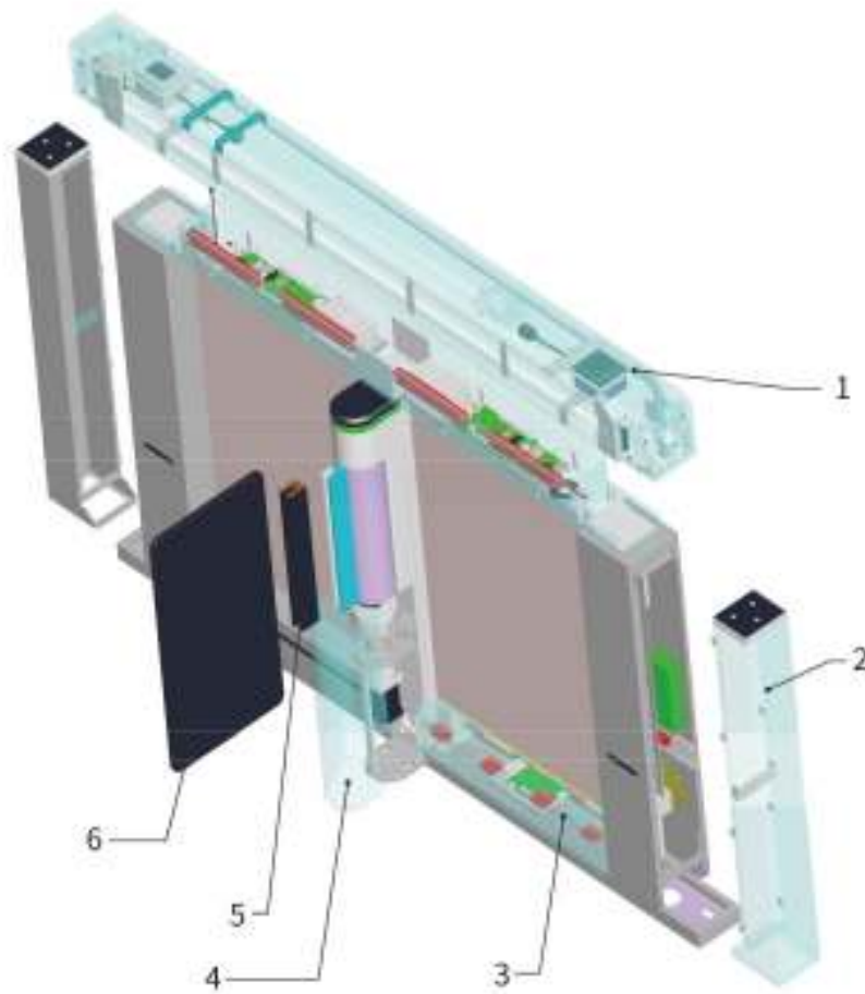
Figure 4-4 Turnstile cabinet doors
