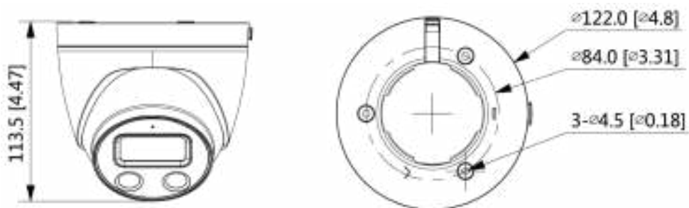
Figure 3-2 Dimension (mm[inch])
