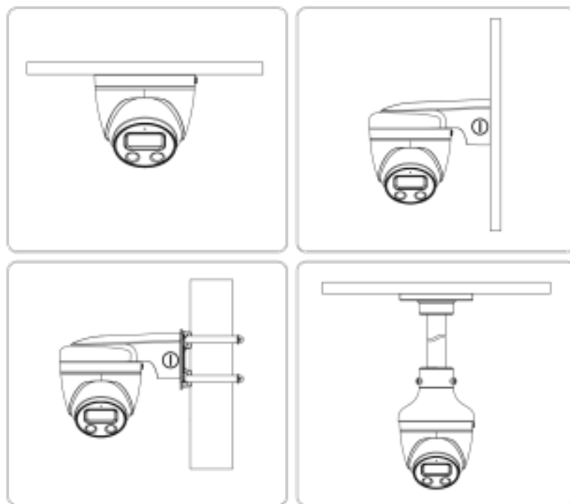
Figure 3-3 Installation type
