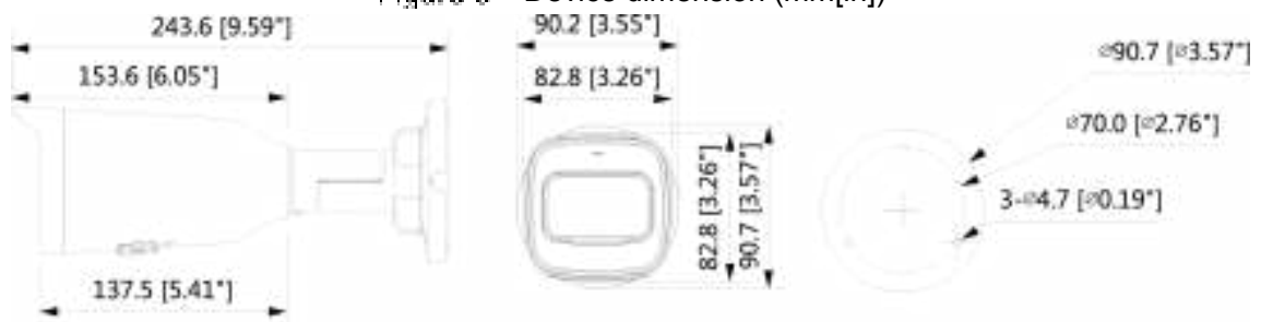
Figure 3- Device dimension (mm[in])
