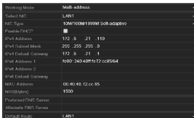
Figure 9.4 Multi-address Working Mode
