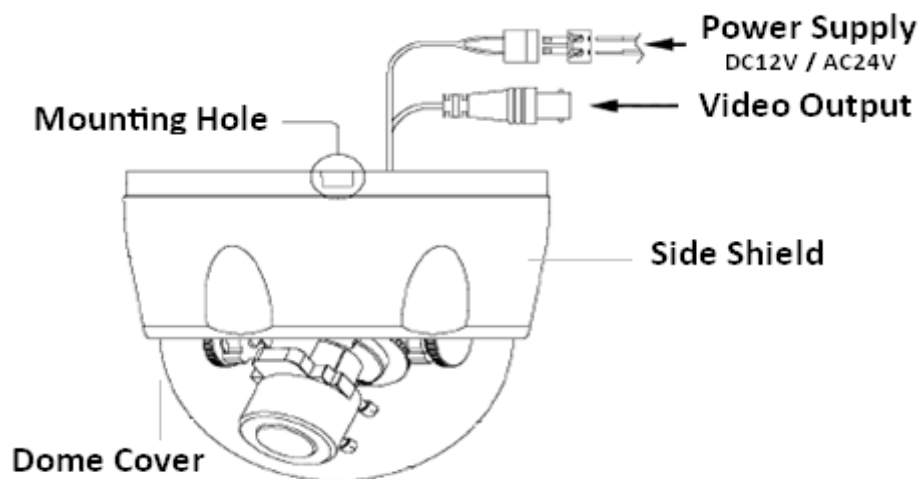
Figure 1.5 DS-2CC511/591P(N)-A
