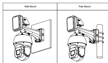
PFA150 Pole Mount Bracket
