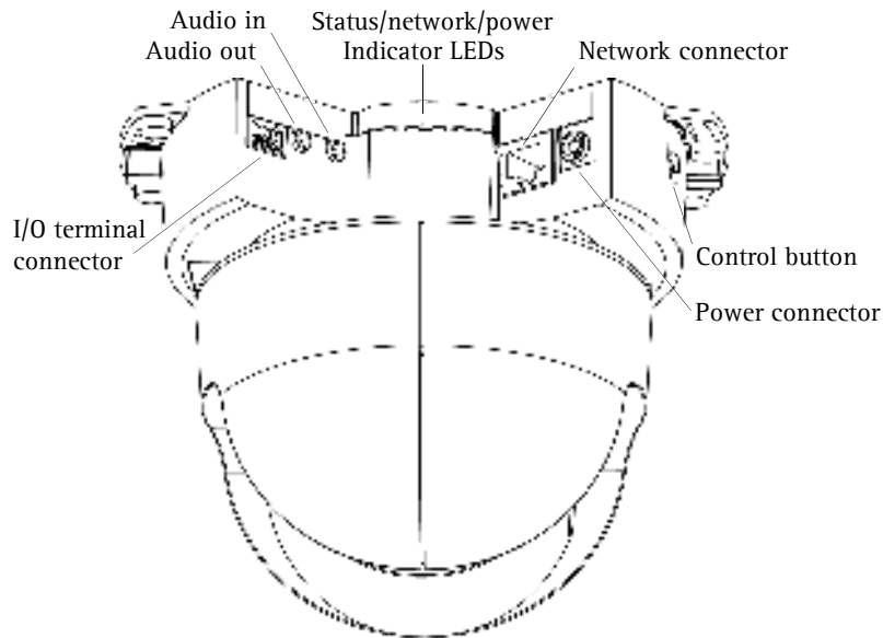
AXIS 215 PTZ Network Camera
