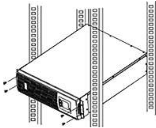
Figure 5. Rackmount installation
