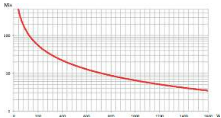
Figure 22. Runtime graph of INFORPRO2000 UPS
