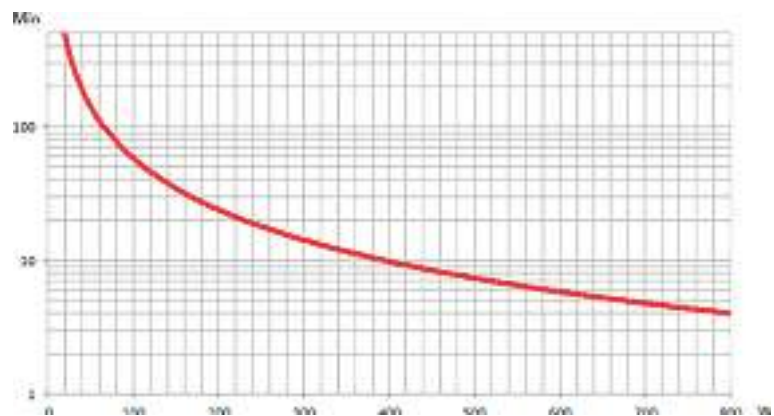
Figure 20. Runtime graph of INFORPRO1000 UPS
