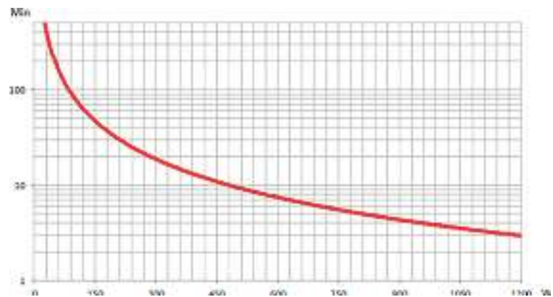
Figure 21. Runtime graph of INFORPRO1500 UPS
