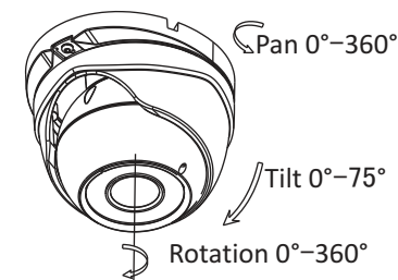
Figure 2-11 Lens Adjustment
