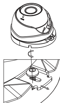
Figure 2-10 The Lock Screw
