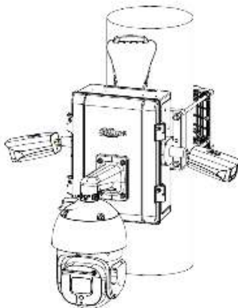
Pole mount
