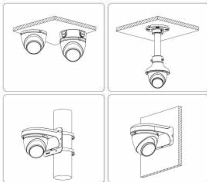
Figure 3-3 Installation method
