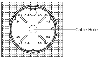
Figure 2-4 Secure the Back box
