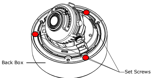
Figure 2-3 Remove the Camera
