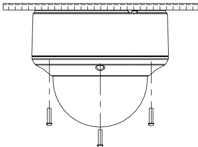
Figure 2-5 Secure Lower Dome
